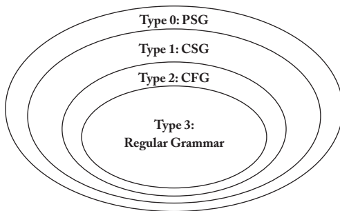
Figure 17.22. Chomsky Hierarchy of Grammars
